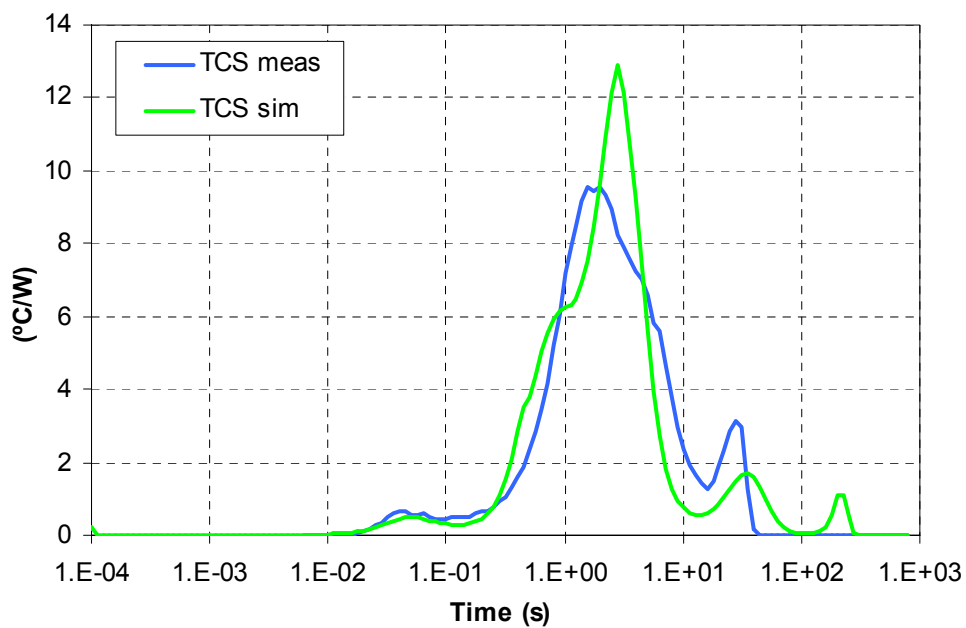
Fig.3.2: DCP4 – TFBGA 12x12 148 - F.C. – Time Constant Spectra
