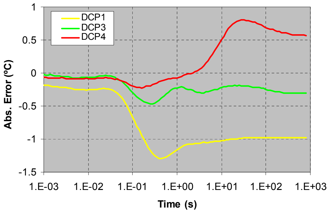
Fig. 4.1: TFBGA12x12, 168 - W.B. – Absolute Error
