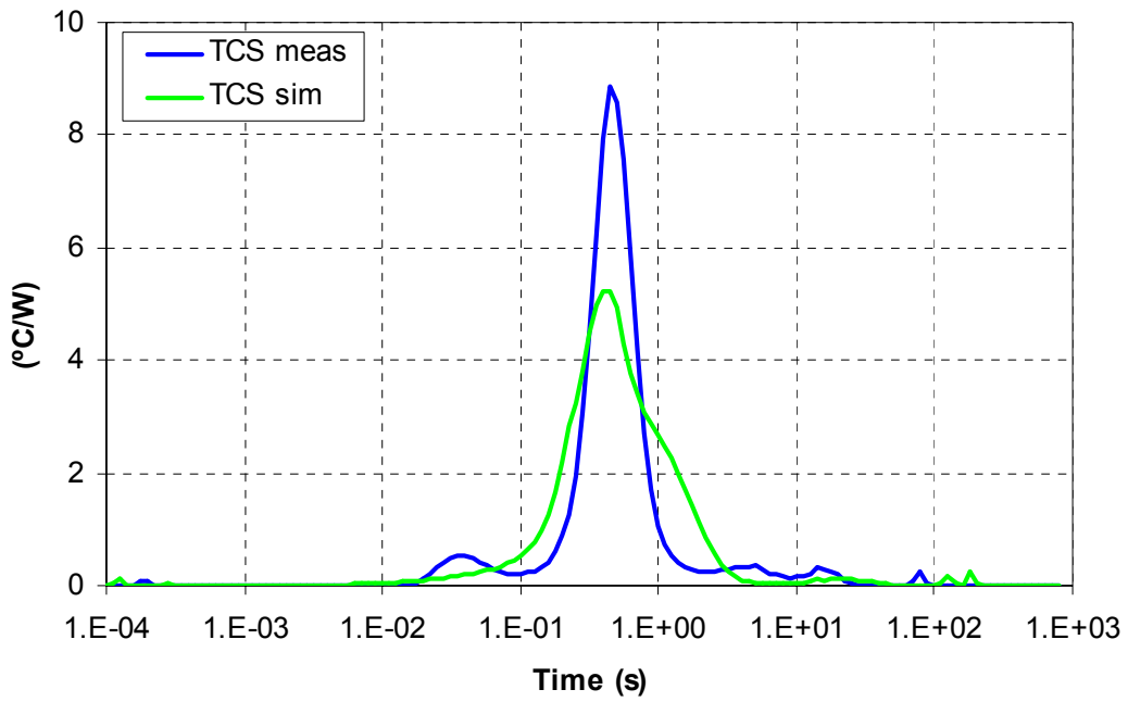
Fig. 2.2: DCP3 – TFBGA 12x12 148 - F.C. – Time Constant Spectra
