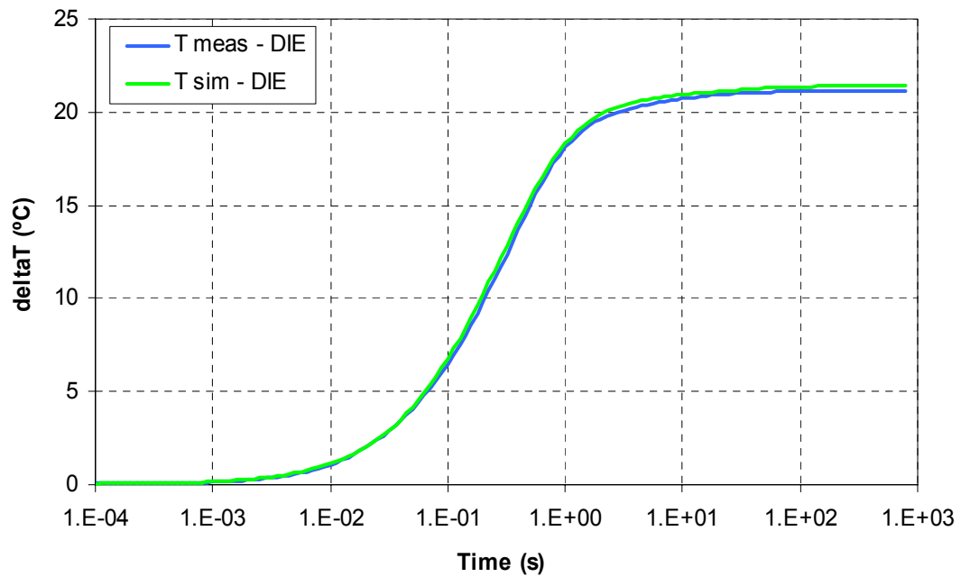
Fig. 2.1: DCP3 – TFBGA12x12, 168 - W.B. – Temperature Curves (P = 2.3 W)
