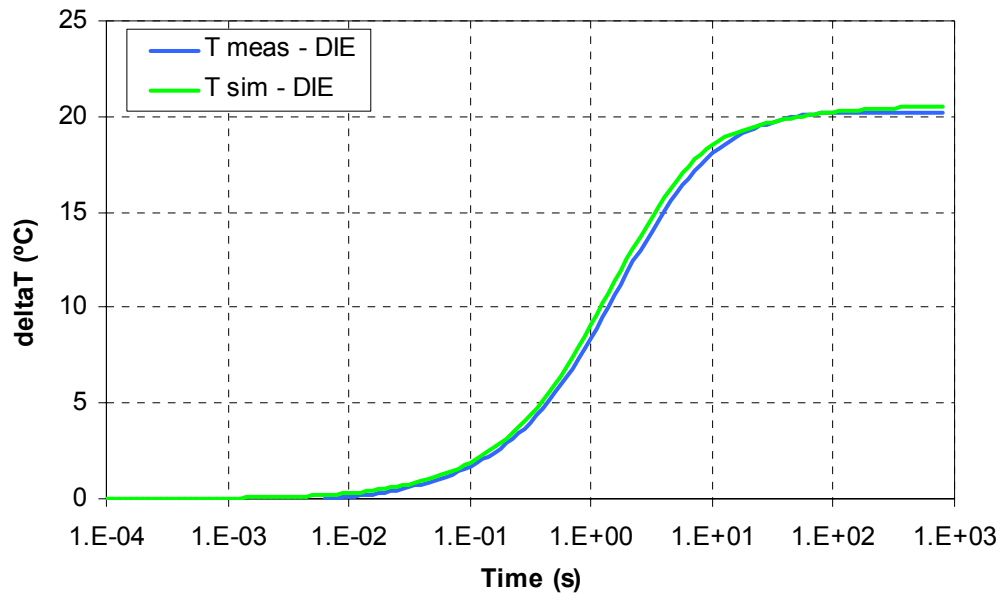
Fig. 3.1: DCP4 – TFBGA 12x12 148 - F.C. – Temperature Curves (P = 0.8 W)
