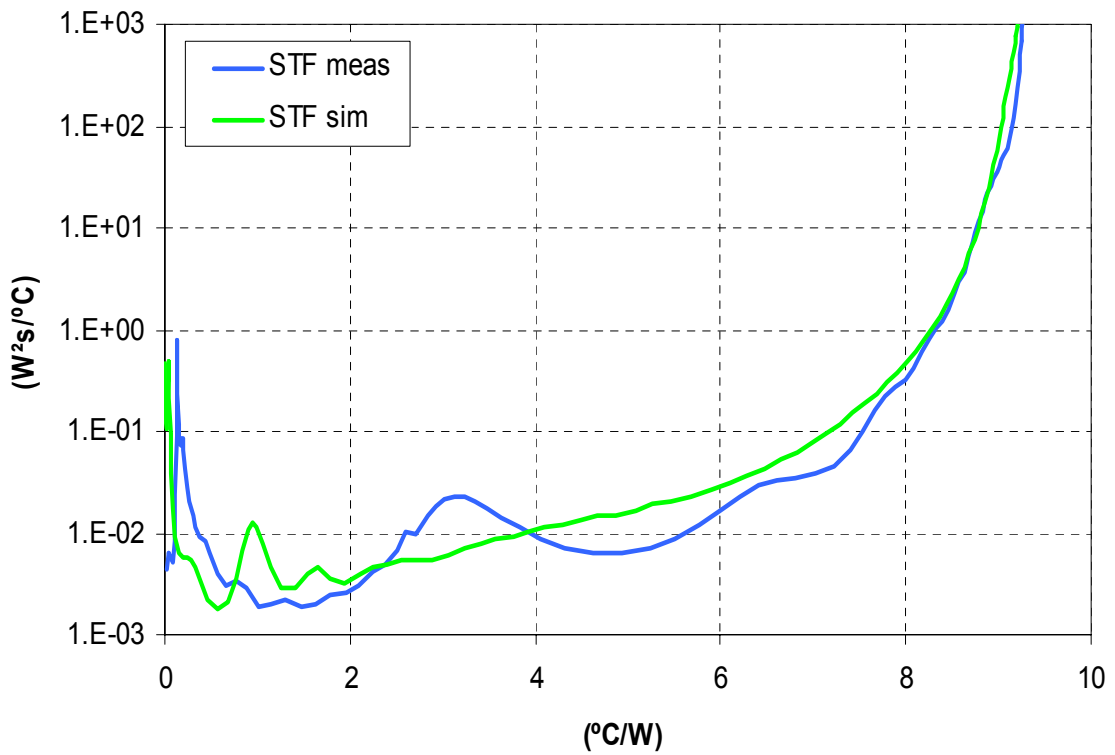
Fig. 2.3: DCP3 – TFBGA12x12, 168 - W.B. – Structure Functions
