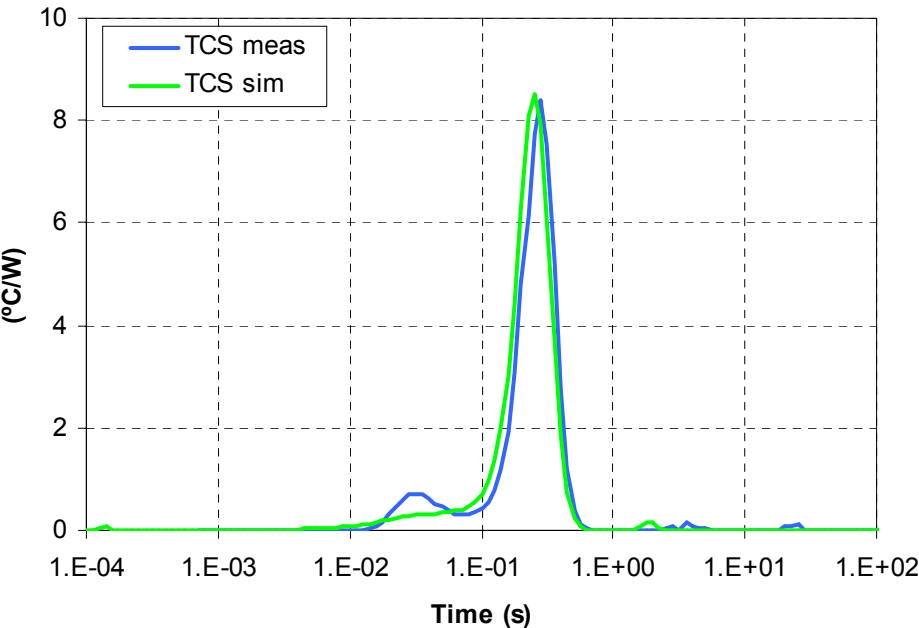
Fig. 1.2: TFBGA12x12, 168 - W.B. – Time Constant Spectra
