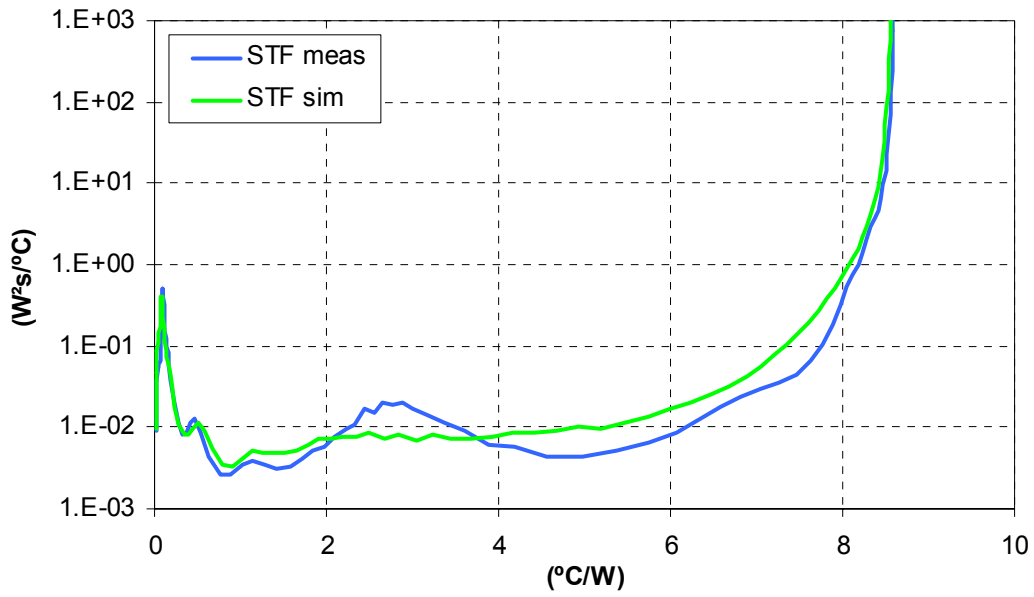
Fig. 1.3: DCP1 – TFBGA12x12, 148 - F.C. – Structure Functions
