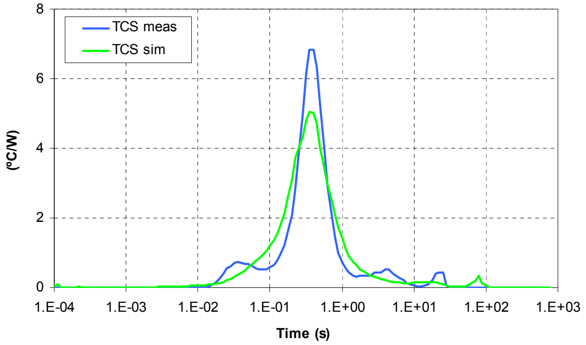
Fig. 2.2: DCP3 – TFBGA12x12, 168 - W.B. – Time Constant Spectra
