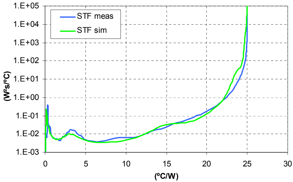
Fig. 3.3: DCP4 – TFBGA 12x12 148 - F.C. – Structure Functions
