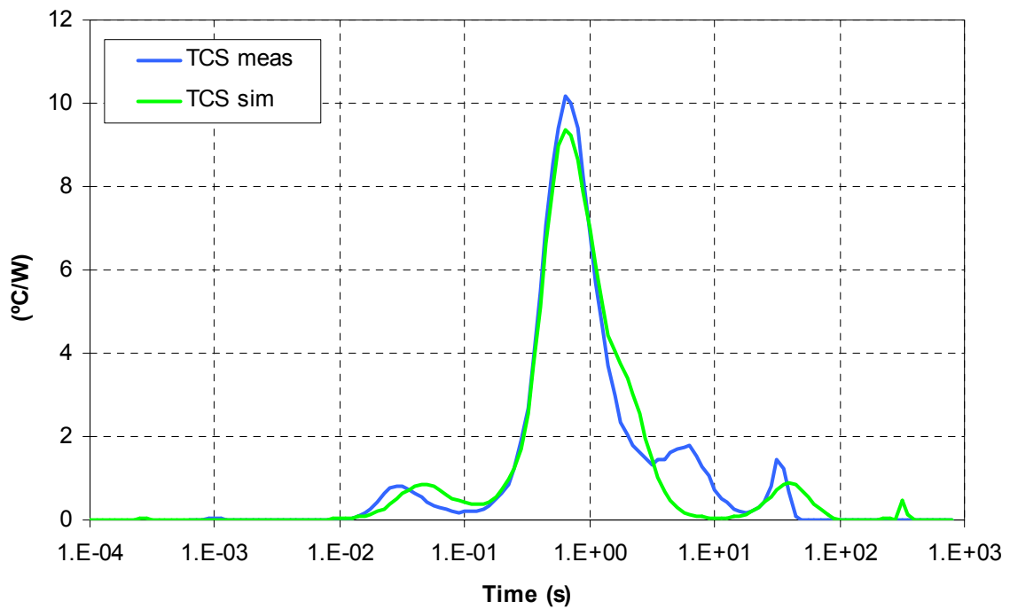
Fig. 3.2: DCP4 – TFBGA12x12, 168 - W.B. – Time Constant Spectra
