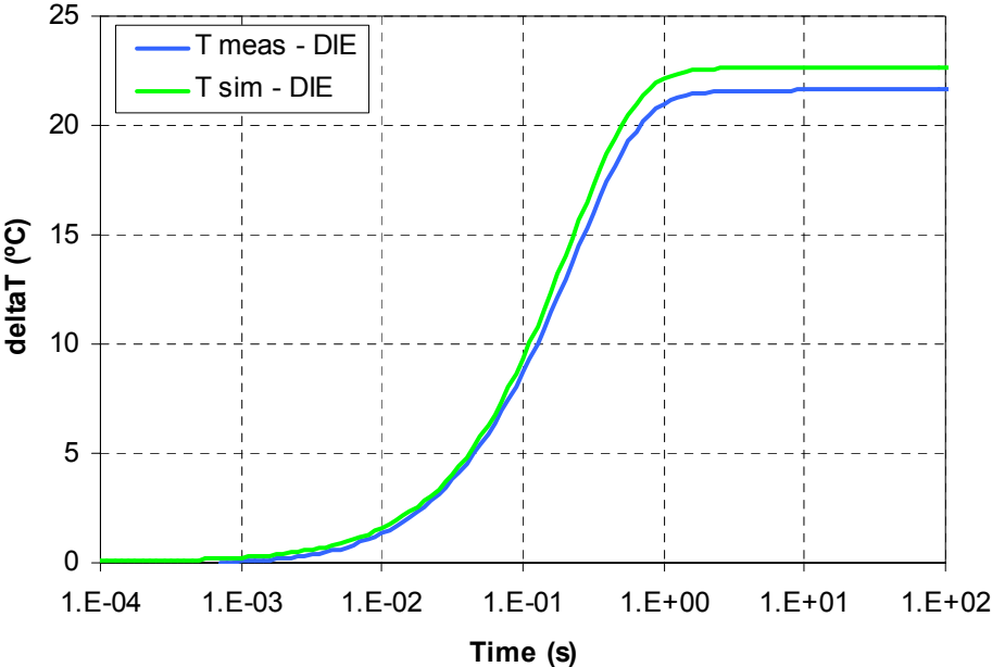
Fig. 1.1: DCP1 – TFBGA12x12, 168 - W.B. – Temperature Curves (P = 3.2 W)
