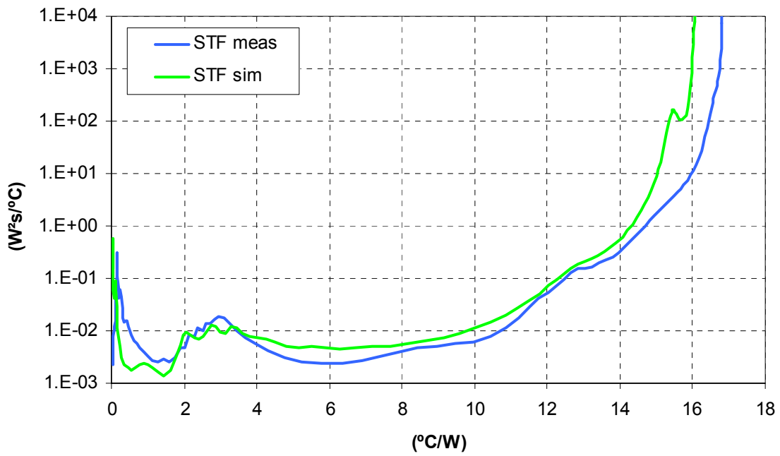
Fig. 3.3: DCP4 – TFBGA12x12, 168 - W.B. – Structure Functions
