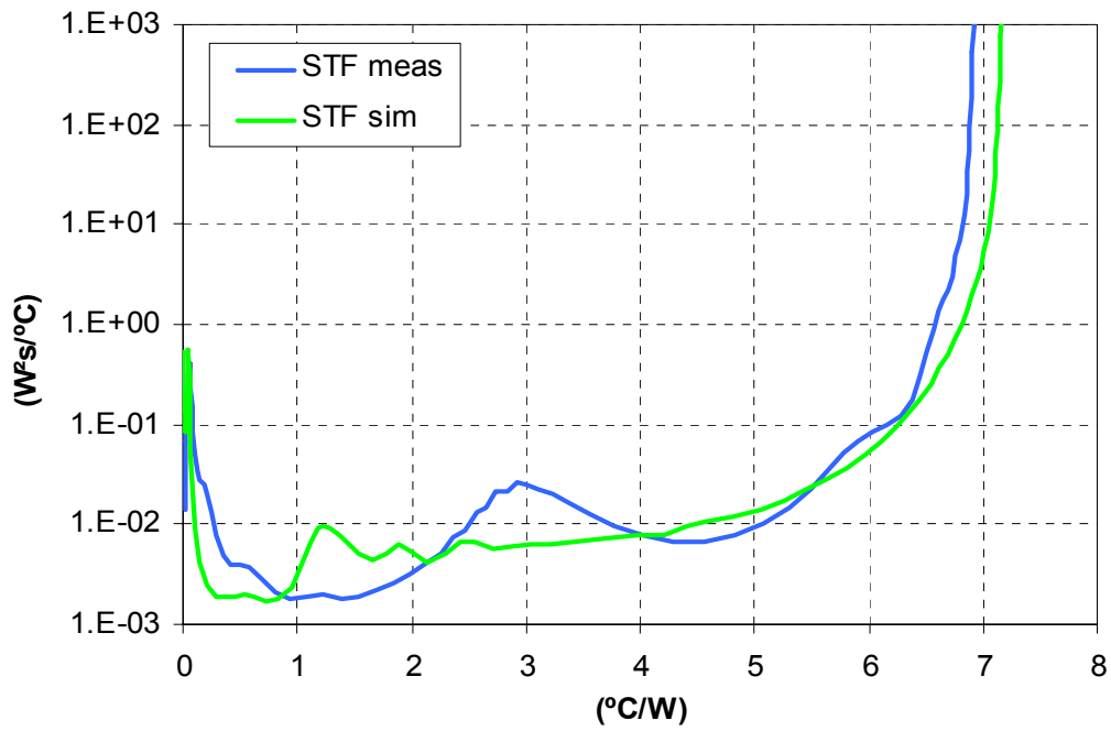
Fig. 1.3: DCP1 – TFBGA12x12, 168 - W.B. – Structure Functions
