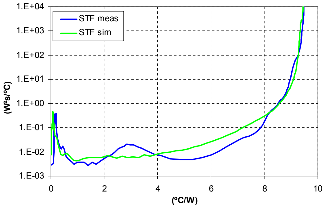
Fig. 2.3: DCP3 – TFBGA 12x12 148 - F.C. – Structure Functions
