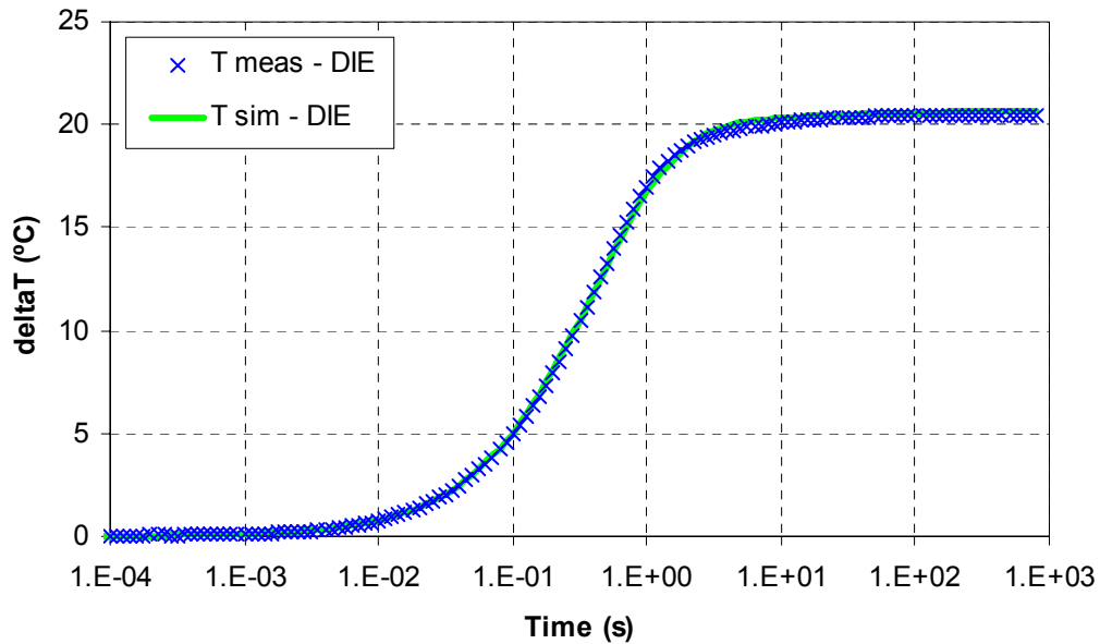
Fig. 2.1: DCP3 – TFBGA 12x12 148 - F.C. – Temperature Curves (P = 2.2 W)
