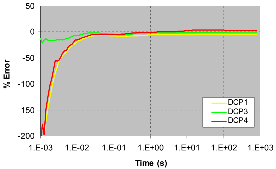
Fig. 4.2: TFBGA12x12, 168 - W.B. – Error (%)
