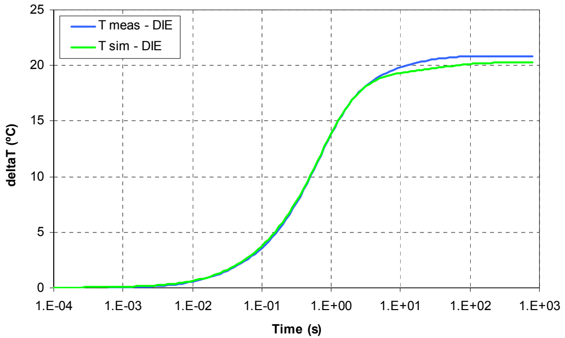
Fig. 3.1: DCP4 – TFBGA12x12, 168 - W.B. – Temperature Curves (P = 1.3 W)
