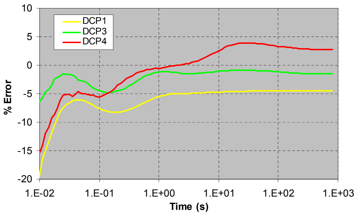
Fig. 4.3: TFBGA12x12, 168 - W.B. – Rescaling fig. 4.2 starting from 10 ms
