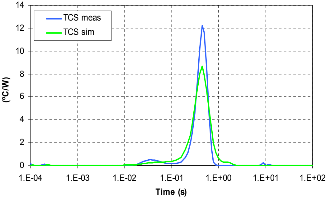
Fig. 1.2: DCP1 – TFBGA12x12, 148 - F.C. – Time Constant Spectra
