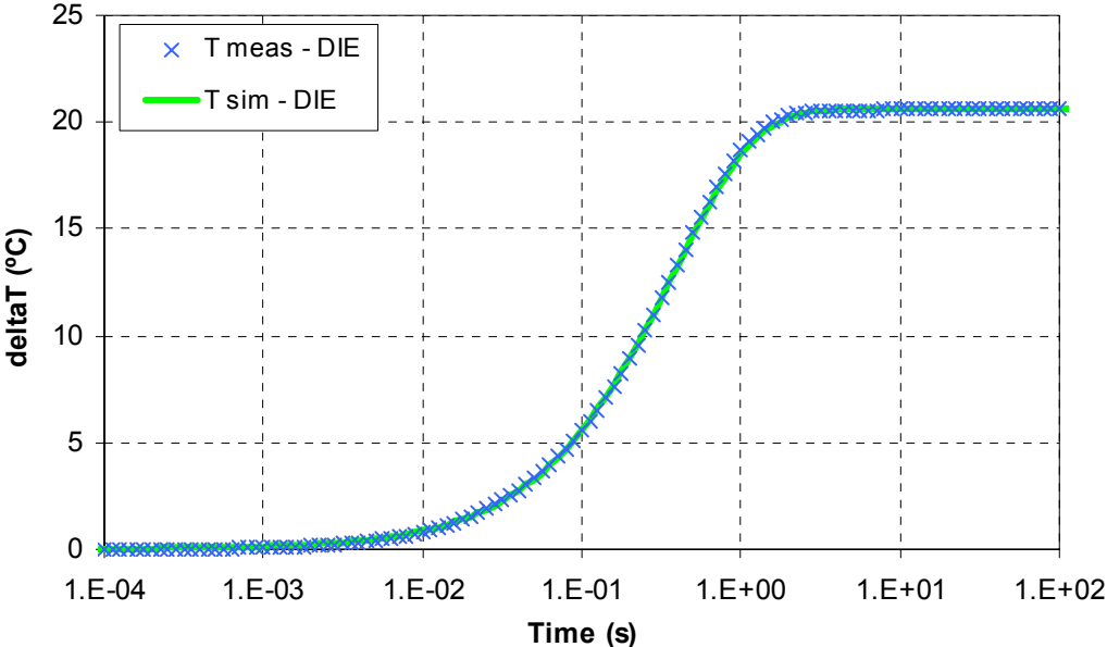
Fig. 1.1: DCP1 – TFBGA12x12, 148 - F.C. – Temperature Curves (P = 2.4 W)
